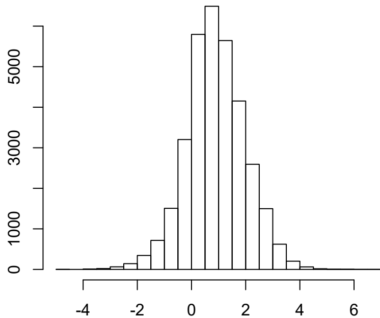
Unconstrained posterior means
