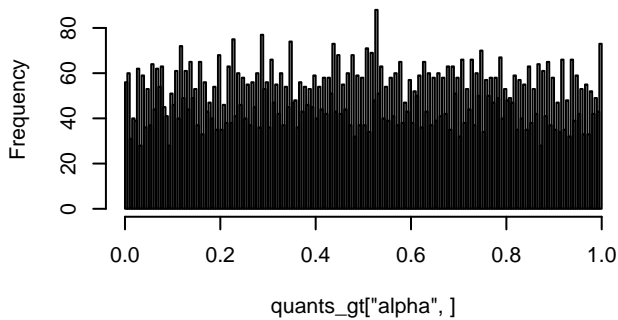
Histogram of quants_gt["alpha", ]
