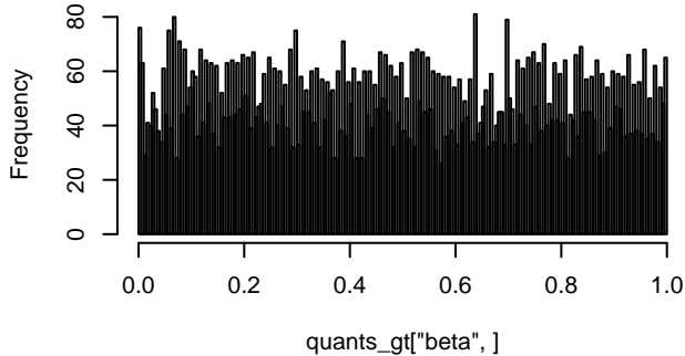
Histogram of quants_gt["beta", ]
