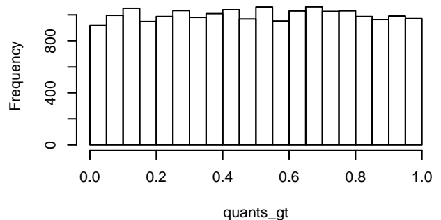
Histogram of quants_gt
