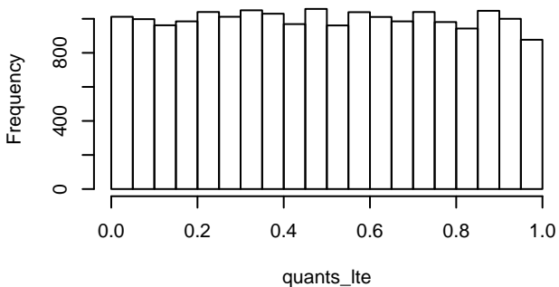
Histogram of quants_lte
