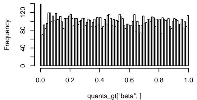
Histogram of quants_gt["beta", ]
