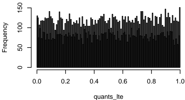
Histogram of quants_lte
