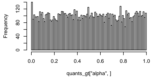
Histogram of quants_gt["alpha", ]
