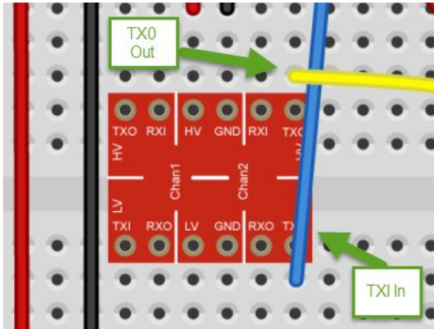
Logic Shifter Connection as per Core Electronics
