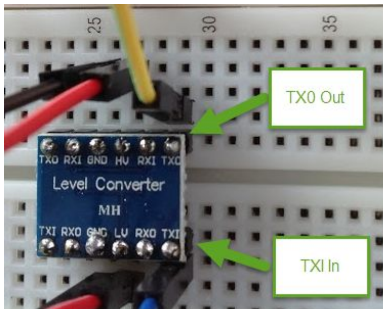
Logic Shifter Connection as per Eddy's Board
